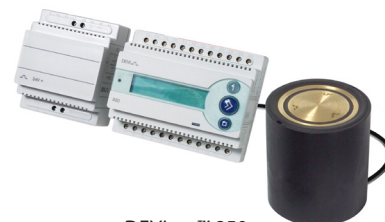
DEVlreg™ 850 with ground sensor
