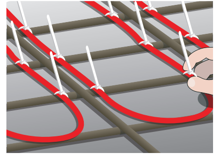
Cable ties
