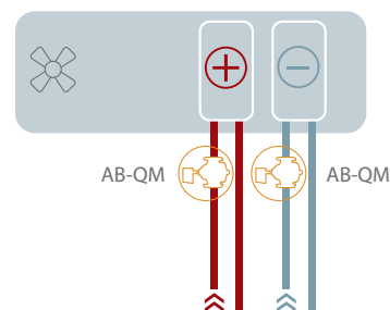
VENTILATIONSAGGREGAT
