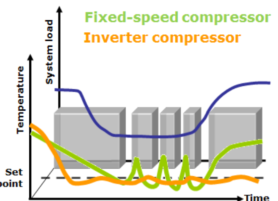
Temperature settings by compressor type
