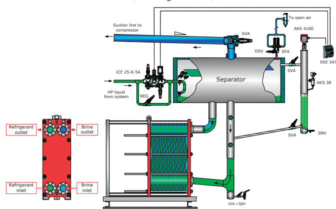
Flooded Evaporator (Cooling of brine)
