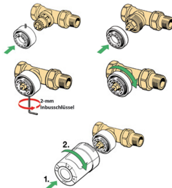
RA-Adapter
