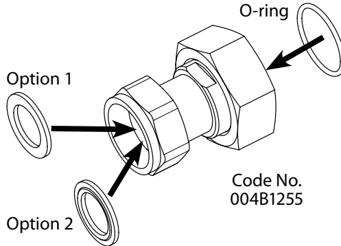
Flat gasket heat exchanger G1A - station with o-ring connection
