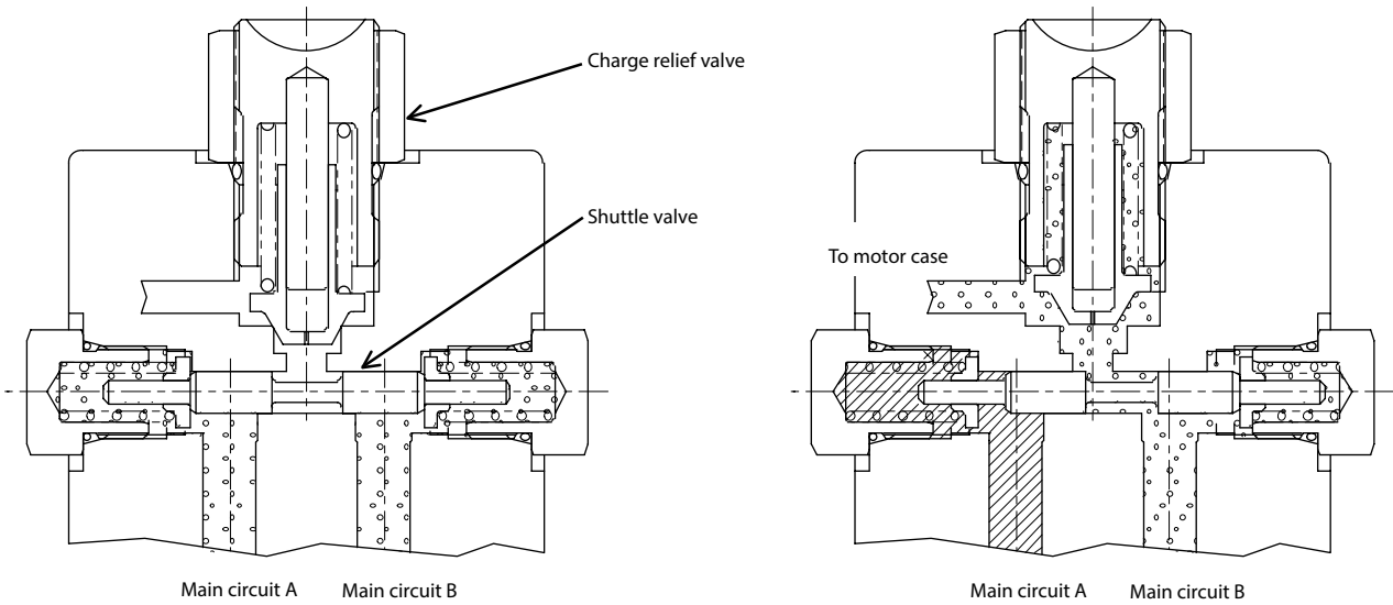
Fig.8 Loop flushing valve
