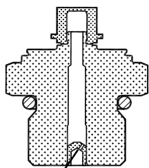
Pulse-snubber
