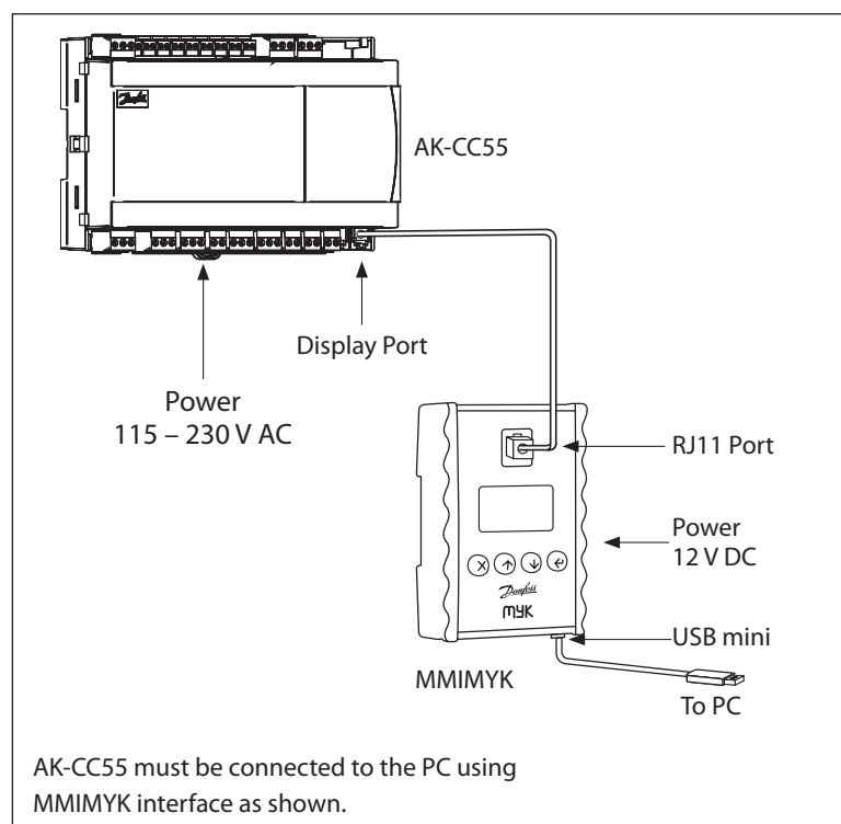
Fig 4. Connection for AK-CC55 using interface type MMIMYK (Code No. 080G0073)
