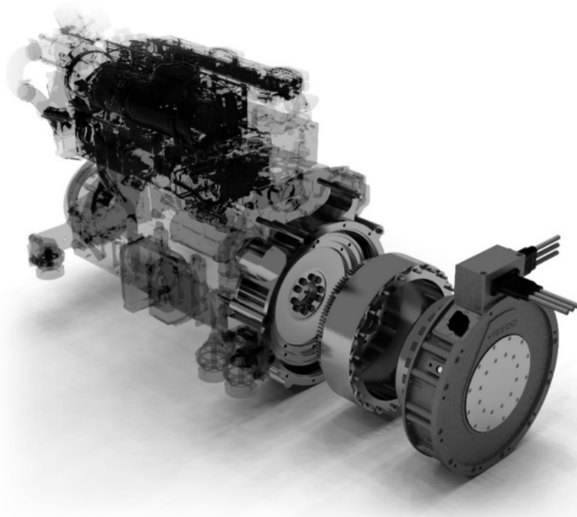
Picture 2 Integrated machine connected to diesel engine flywheel housing
