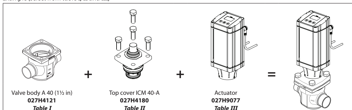
ICV 40 valve body w/different connections
