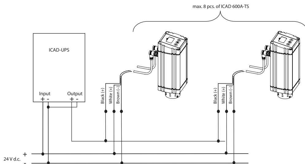
One 24 V DC tranformer for ICAD-UPS and ICAD 600A-TS
