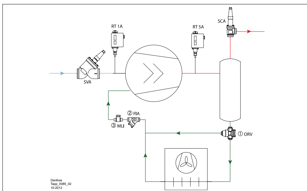
Example of the system with ORV for diverting operation
