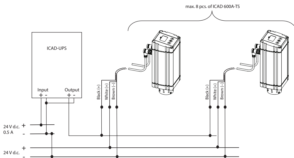
Seperate 24 V DC tranformer for both ICAD-UPS and ICAD 600A-TS
