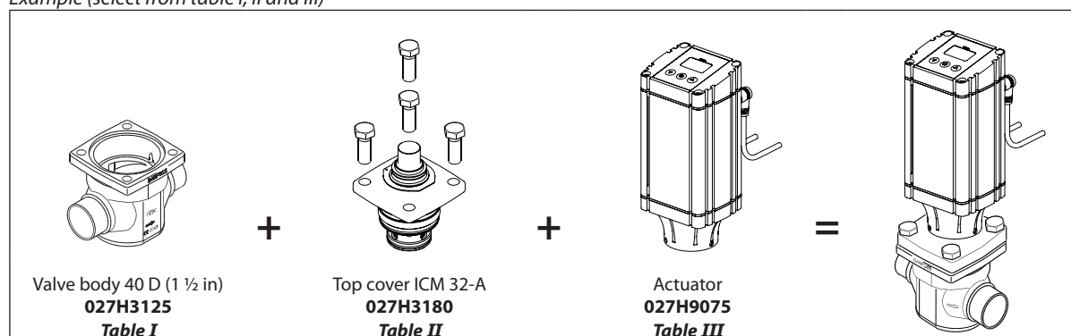
ICV 32 valve body w/different connections
