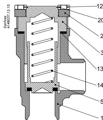
CHV-SS 15 - 40 (1/2" - 1 1/2")
