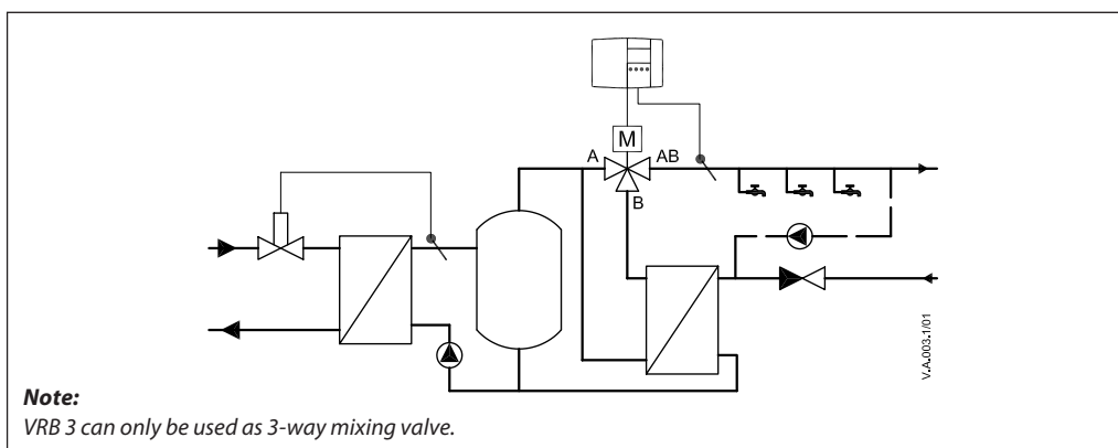
Fig. 1 Mixing valve used in mixing application.
