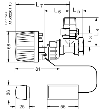
Angle valve with thermostatic sensor RA2992
