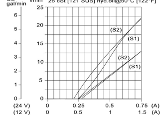
Operating curves with R16 coil and steel nut Pressure drop of circuit 10 Bar. 26 cSt [121 SUS] hyd.oil@50°C [122°F]
