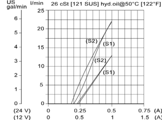
Operating curves with R16 coil and steel nut Pressure drop of circuit 10 Bar. 26 cSt [121 SUS] hyd.oil@50°C [122°F]
