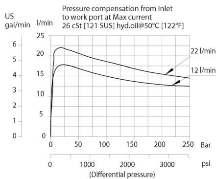
Operating curves with R16 coil and steel nut Pressure drop of circuit 10 Bar. 26 cSt [121 SUS] hyd.oil@50°C [122°F]
