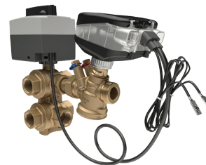
6-way valve + PICV: NovoCon ChangeOver6 +AB-QM
