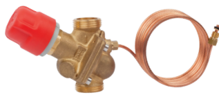
ABV: AB-PM +TWA-Q (optional)
