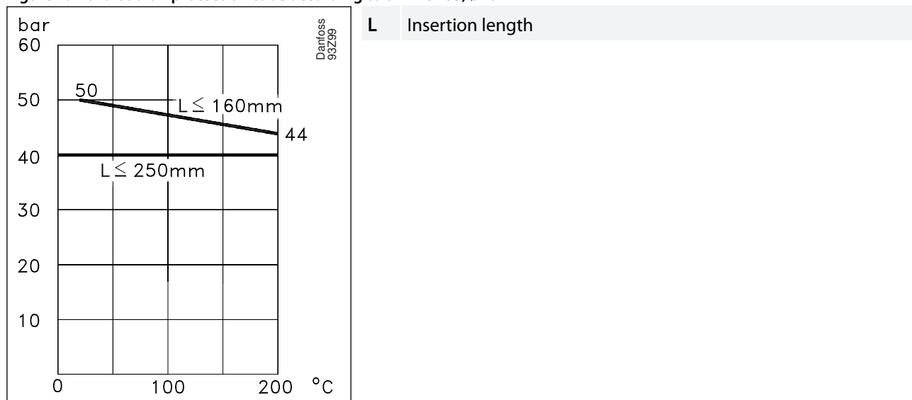
Figure 1: Max. load on protection tube according to DIN 43763, \phi 10 \times 2
