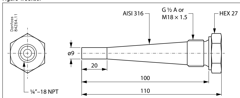
Figure 4: Sensor
