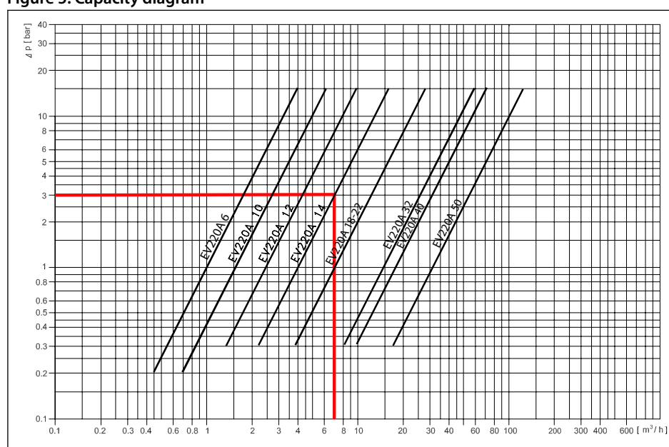
Figure 5: Capacity diagram
