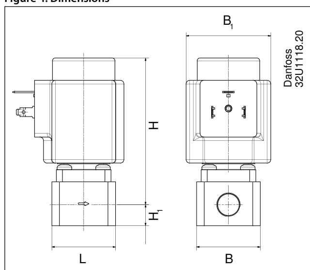
Figure 4: Dimensions
