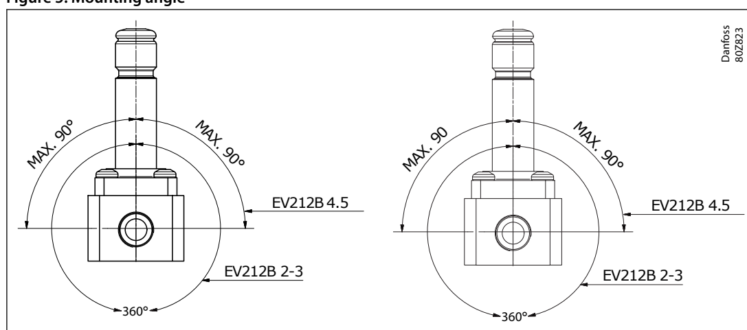
Figure 5: Mounting angle
