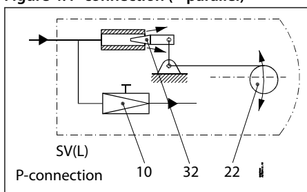
Figure 4: P-connection (= parallel)
