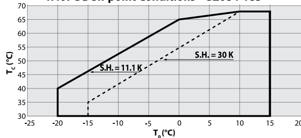
R407C Dew point Conditions - SZ084-185
