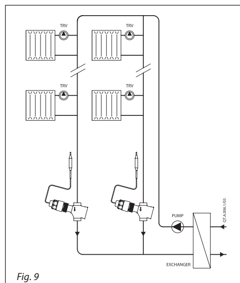
Fig. 9 “Typical one-pipe riser with AB-QM 4.0 & QT installed”
