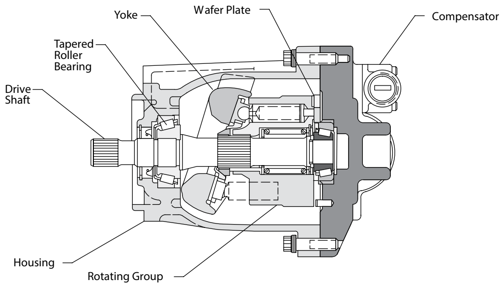
PVE012 Section V iew
