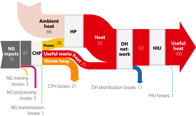
Figure 4. Energy flow diagram for the blue district heating scenario.
