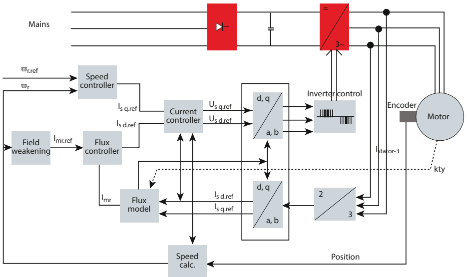
Fig. 3.25 Structure of closed loop flux vector control
