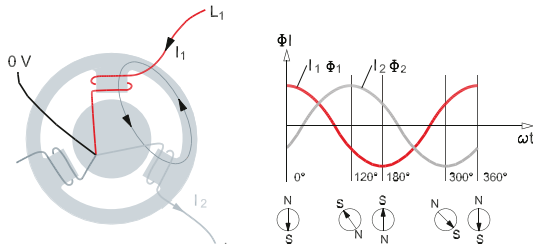
Fig. 2.8 Two phases produce an asymmetrical rotating field
