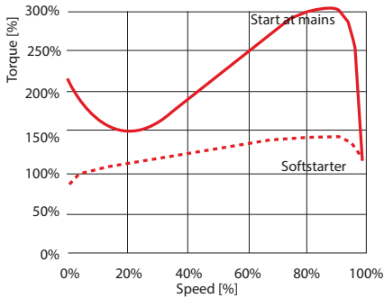
Fig. 4.11 Comparison of motor start direct on mains with motor started by a softstarter (400% current limit)
