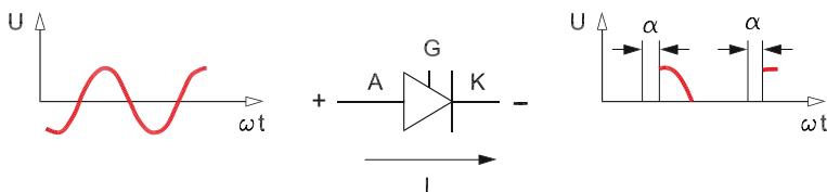
Fig. 3.6 How thyristors work
