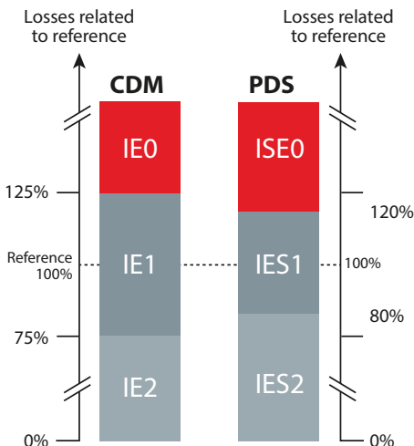
Fig. 5.7 Definition of CDM and PDS efficiency classes
