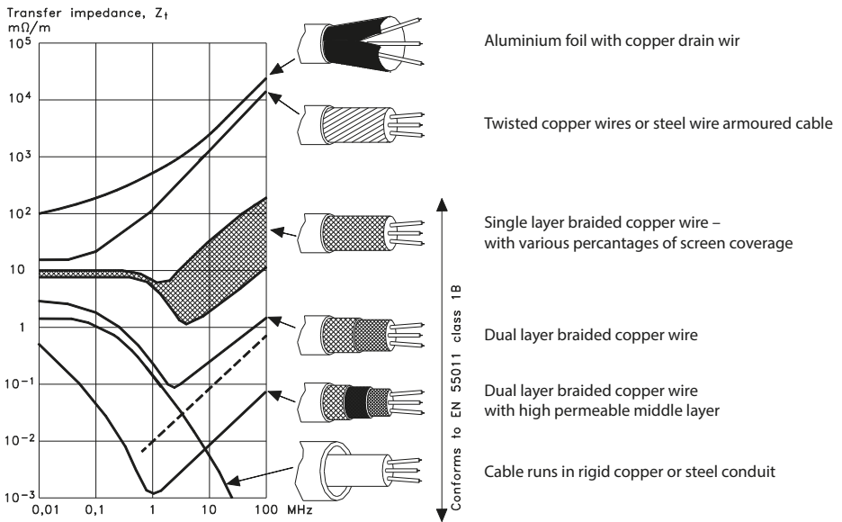
Fig. 6.6 Shielding performance of different cable types
