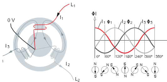
Fig. 2.9 Three phases produce a symmetrical rotating field
