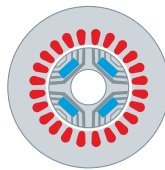
Fig. 2.34 The PM assisted SynRM motor has small magnets inserted in the lamination
