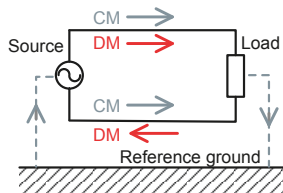
Fig. 6.2 Common-mode and differential-mode
