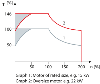
Fig. 4.18 T/n characteristics with and without external cooling
