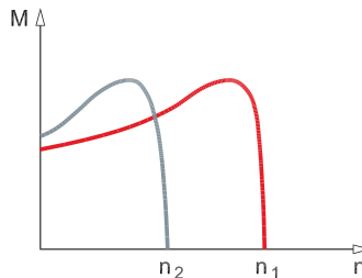
Fig. 2.17 Torque characteristics when changing pole number
