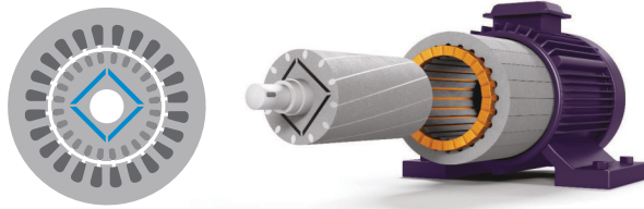
Fig. 2.27 The position of magnets in the rotor influences the motor characteristics
