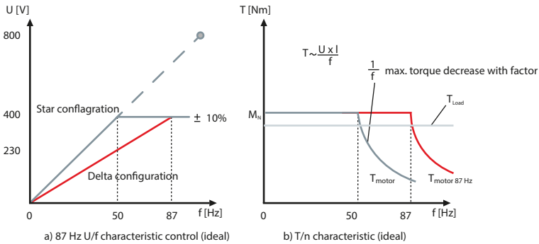
Fig. 4.2 87 Hz characteristic
