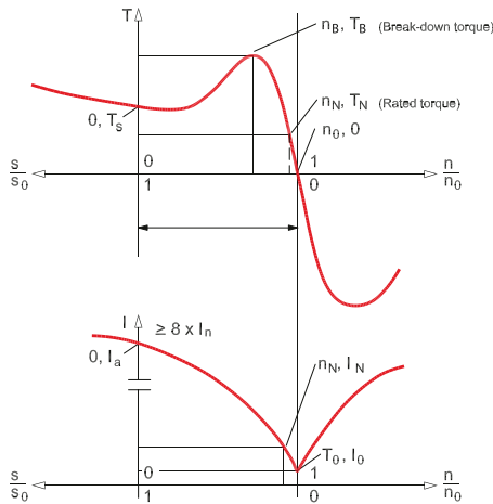
Fig. 2.14 Principal motor current and torque characteristics
