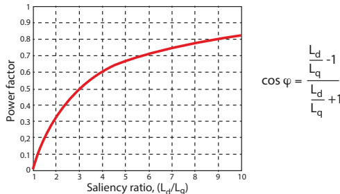
Fig. 2.29 Maximum power factor vs. saliency ratio
