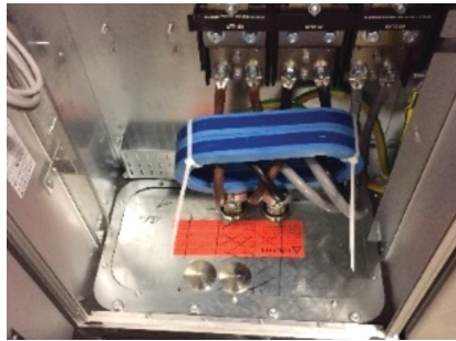
Fig. 6.21 Common-mode cores installed at the drive terminals
