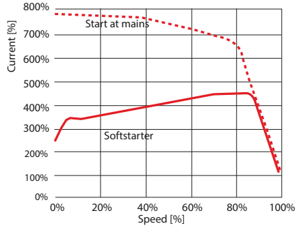
Fig. 4.11 Comparison of motor start direct on mains with motor started by a softstarter (400% current limit)
