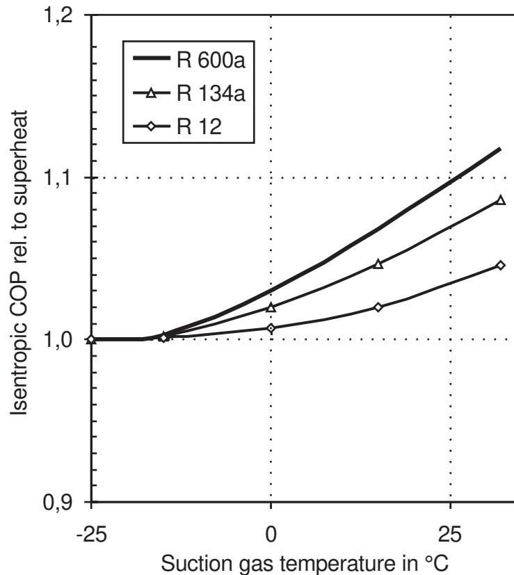
Figure 6: Theoretical COP increase of different refrigerants versus suction temperature with adiabatic compression, internal heat exchange, at -25 °C evaporation, 55 °C condensation, no subcooling before internal heat exchanger
