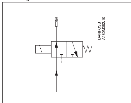
Coil energized
