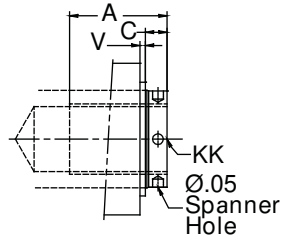
Type #4 Short Female UN Thread
