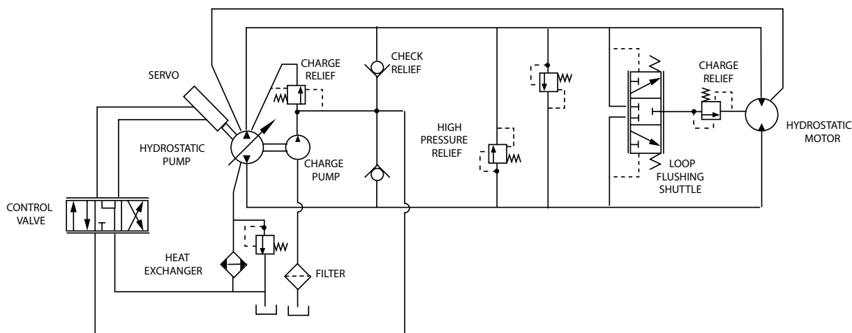
Typical Closed Circuit Transmission Schematic
