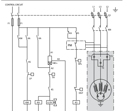
Wiring diagram with pump-down cycle
