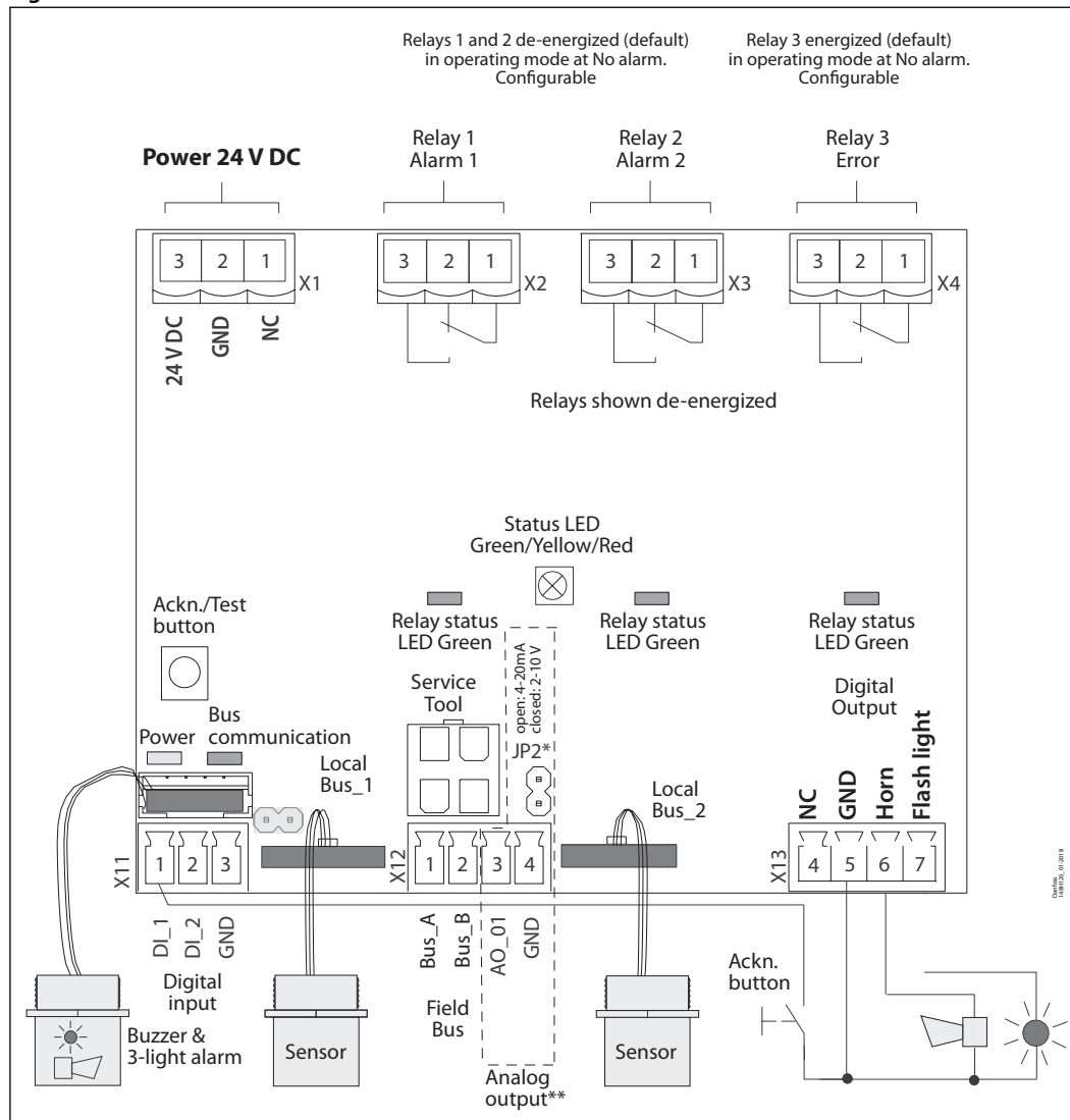
Figure 2: Electrical connection
