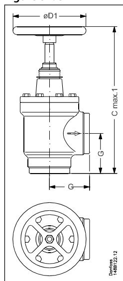
Figure 30: SVA-xx x x ANG CAP Figure 31: SVA-xx x x ANG H-WHEEL
