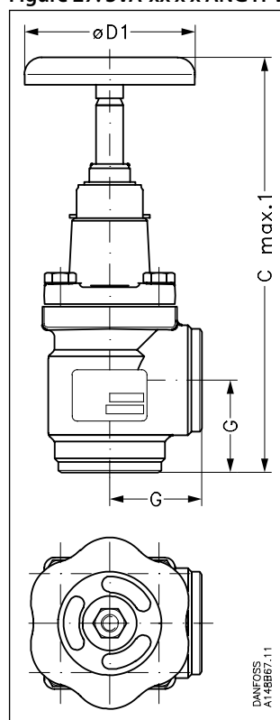
Figure 27: SVA-xx x x ANG H-WHEEL
