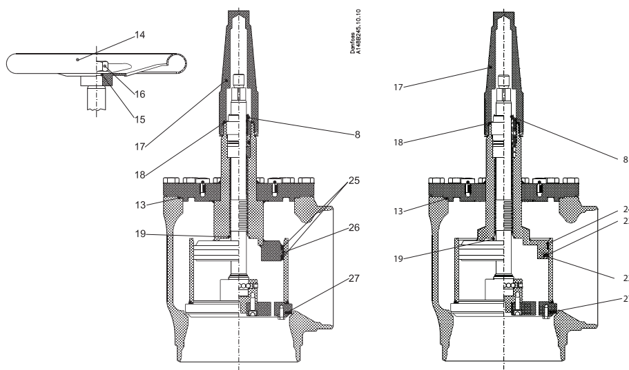
SVA-DH (with u-sleeve gasket for cone)
