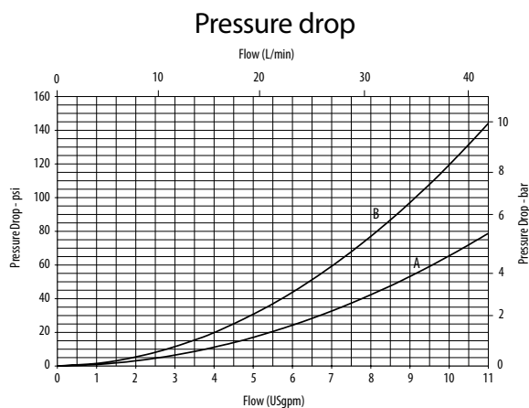
A-Port 1 to 2 • B-Port 3 to 1
