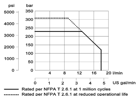
Operating envelope
