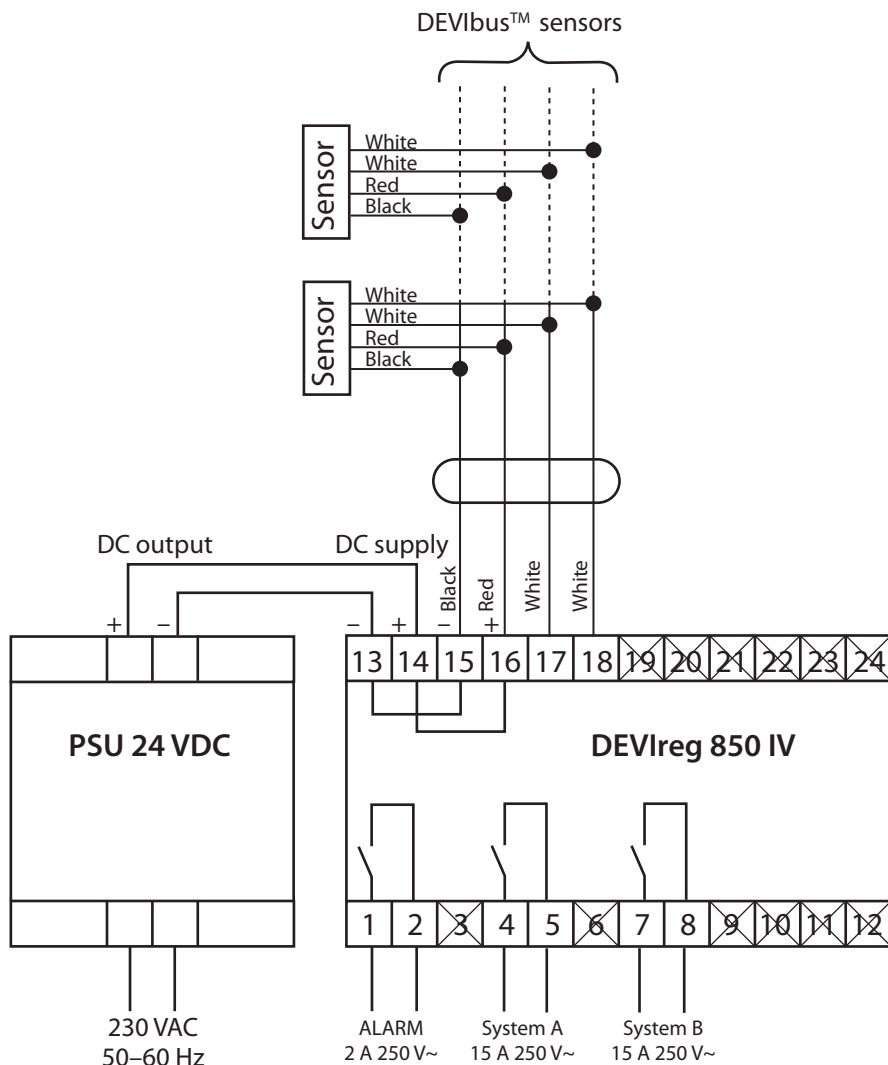
Fig. A — Connection of DEVIreg™ 850 IV
