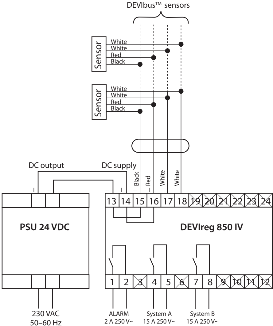
Fig. A — Connection of DEVIreg™ 850 IV
