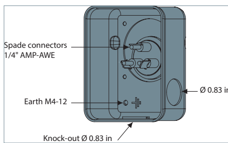
Terminal box for model (1)
