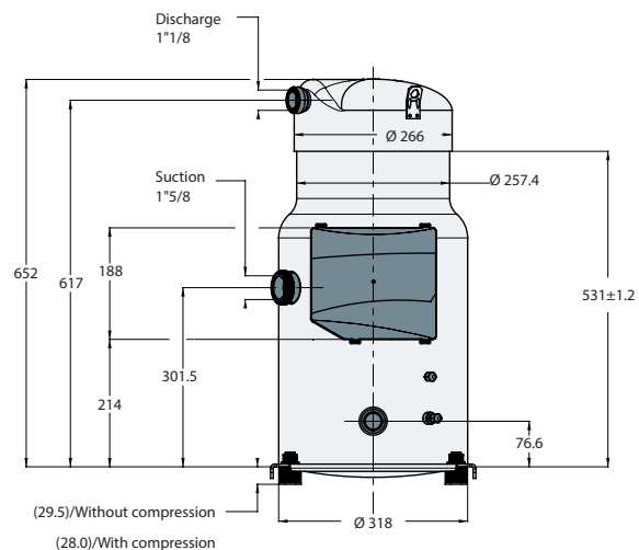
Rotolock connection-MLZ/MLM116 T4QC5
