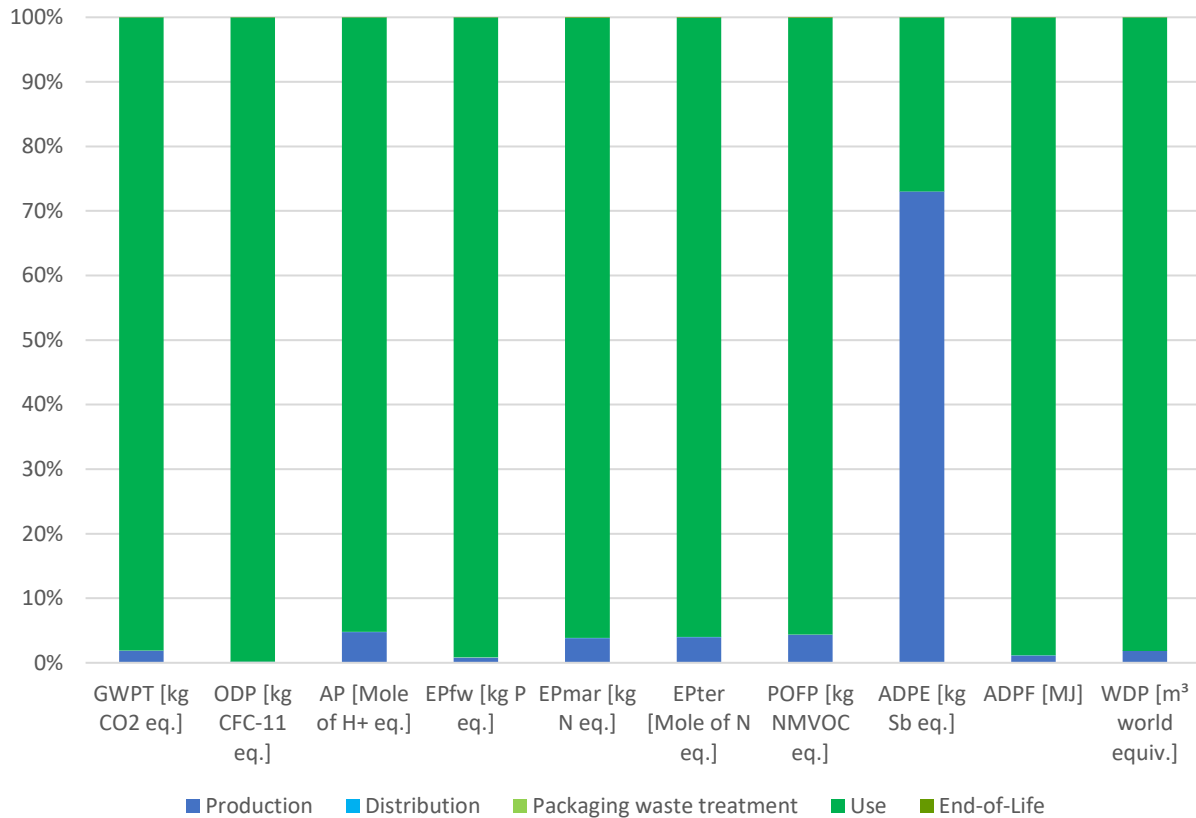
Figure 4: Breakdown of environmental impacts by life cycle stages (see Table 6 for descriptions of environmental impact indicators).
