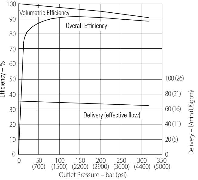
Delivery and Efficiency at 1200 r/min
