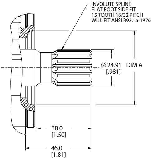
08 - SAE J744-25-4, SAE B-B, 15T SPLINE
