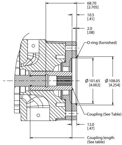
With adapter plate
