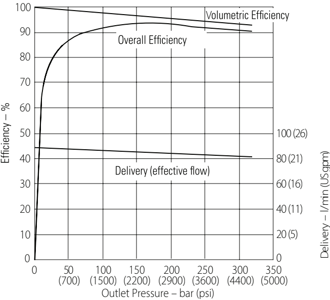
Delivery and Efficiency at 1500 r/min
