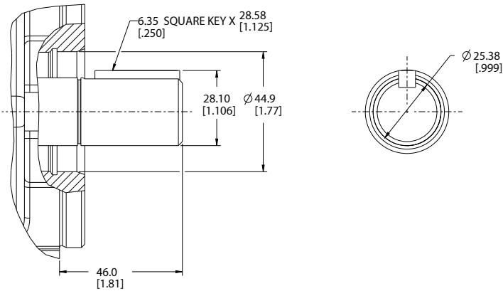
06 - SAE J744-25-1, SAE B-B, STRAIGHT KEYED
