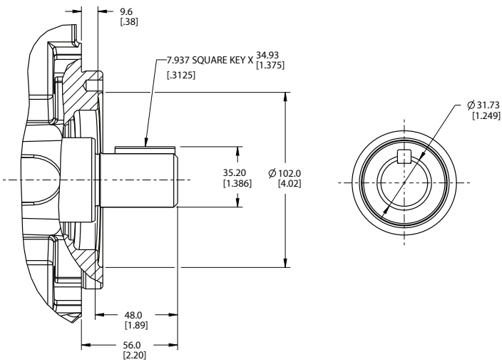
09 - SAE J744-32-1 SAE C STRAIGHT KEYED
