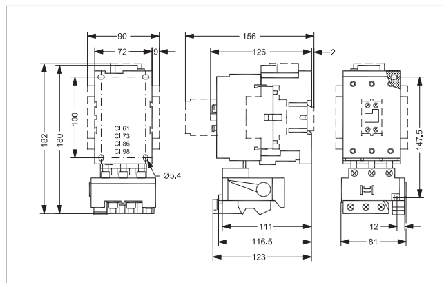
Contactor CI 61, 73, 86, 98 built together with thermal overload relay TI 80-86
