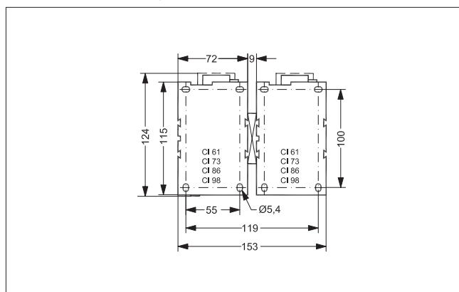
Thermal overload relays TI 80 and TI 86 for contactors CI 61, 73, 86
