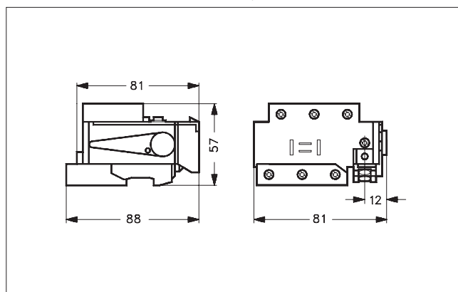
Thermal overload relays TI 80 and TI 86
