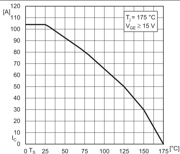
Fig. 2: Rated current vs. temperature I_C = f(T_s)
