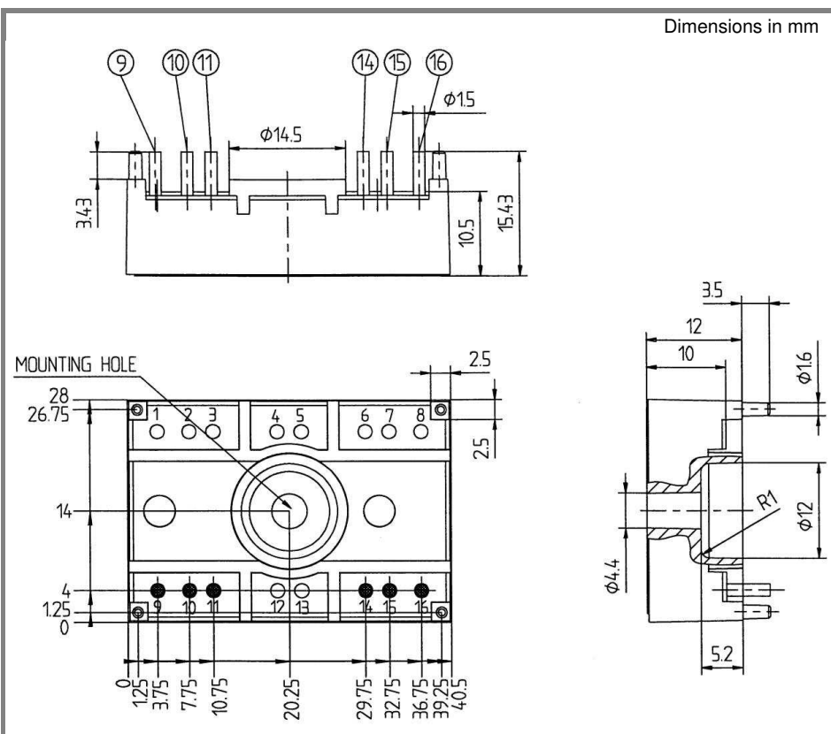
Case T 2 (Suggested hole diameter in the PCB for solder pins and mounting pins : 2mm)
