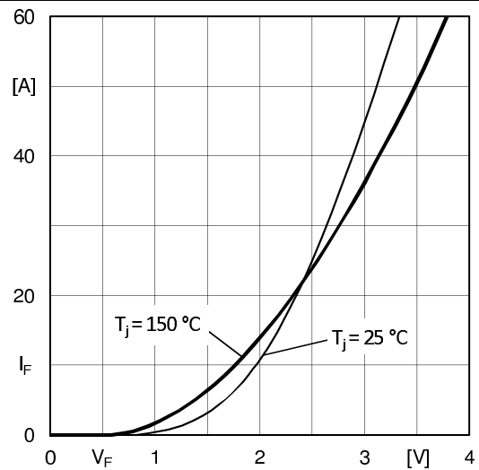
Fig. 10: Typ. CAL diode forward characteristic
