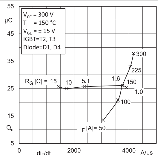
Fig. 24: Typ. Diode1 recovery charge
