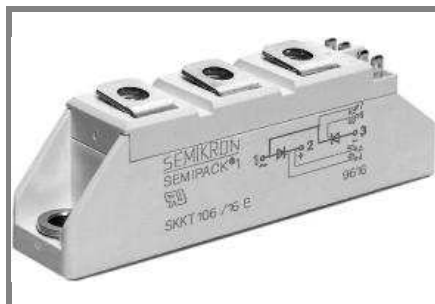
SEMIPACK® 1
