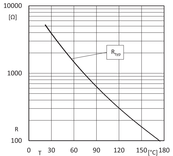
Fig. 26: Typ. NTC characteristics
