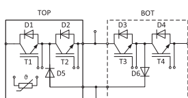
MLI TOP-Switch
