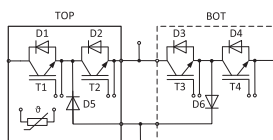
MLI TOP-Switch
